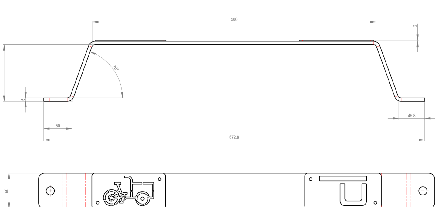
Figure 3 : dimensions rack cargo
