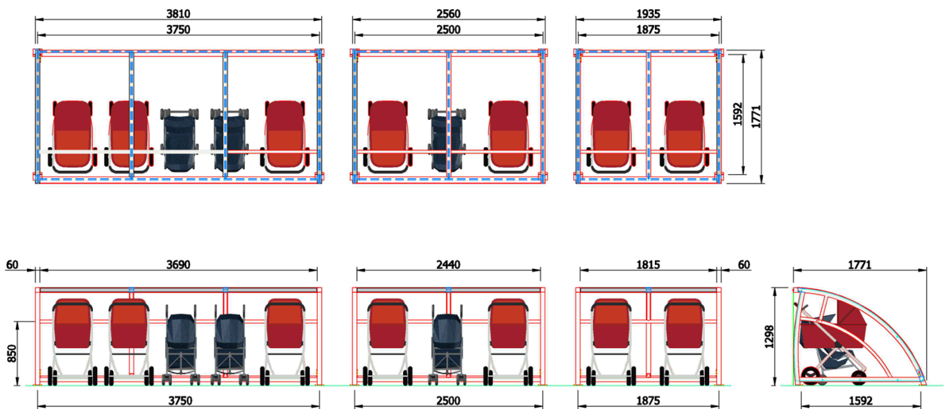
Figure 3. Dimensions modules
